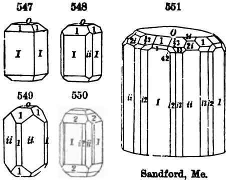
Sandford, Me.
